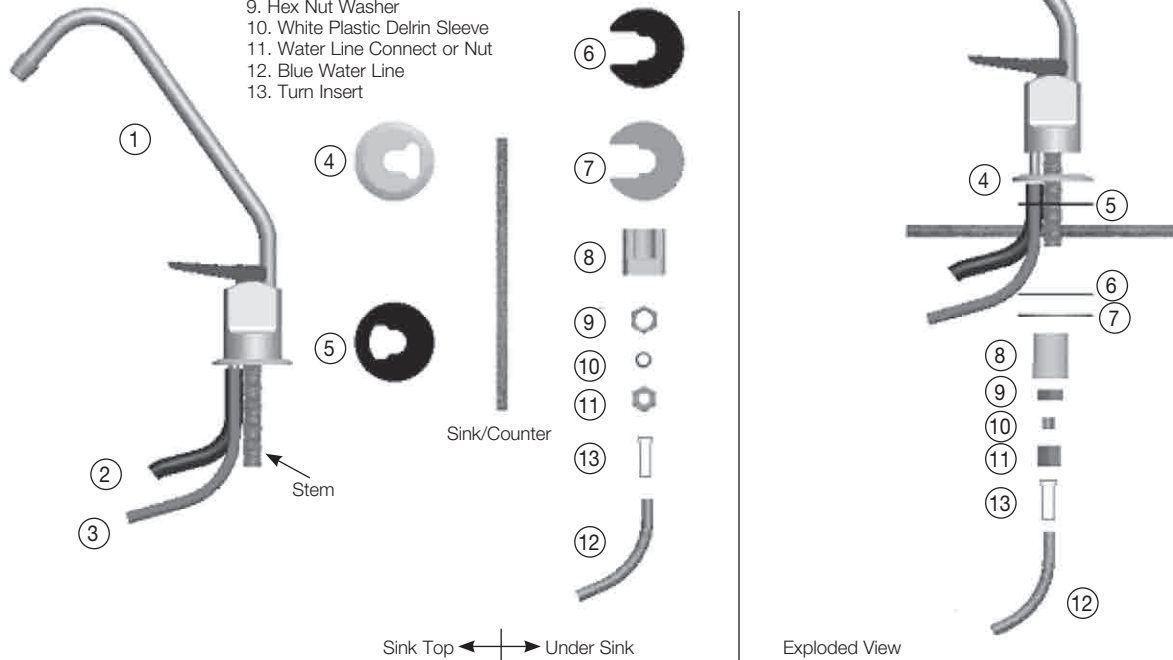
1. List of Parts and Assembly in Exploded View
